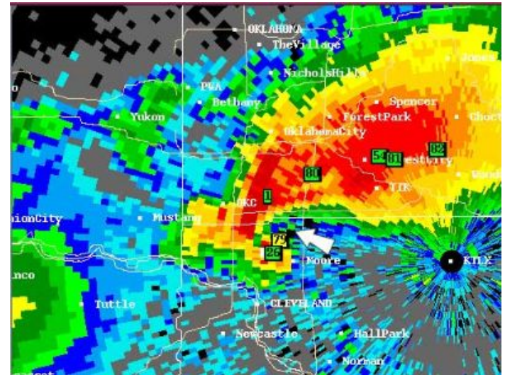
NEXRAD radar reflectivity image, NSSL
